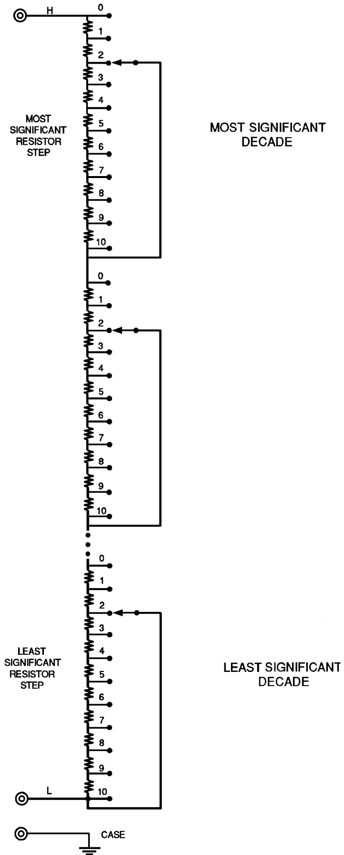
Figure 4.1. HARS Series Schematic Diagram
